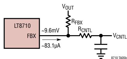
Schematic and Equations for Calculating V_{OUT}
