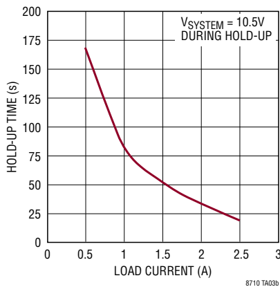
System Hold-Up Time vs System Load Current
