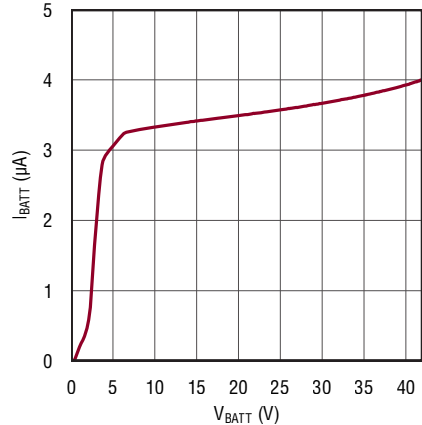
Total Input Current in Shutdown
