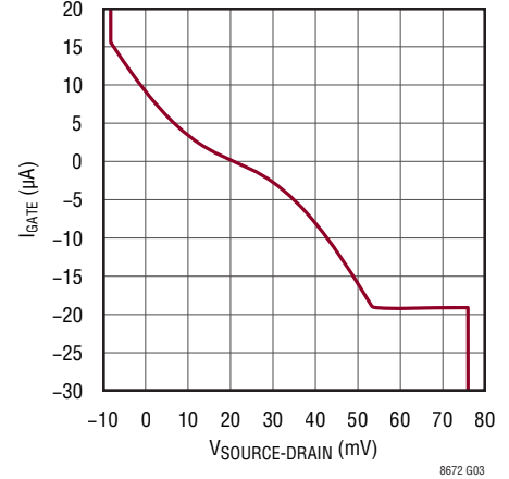
GATE Current vs Forward Voltage Drop
