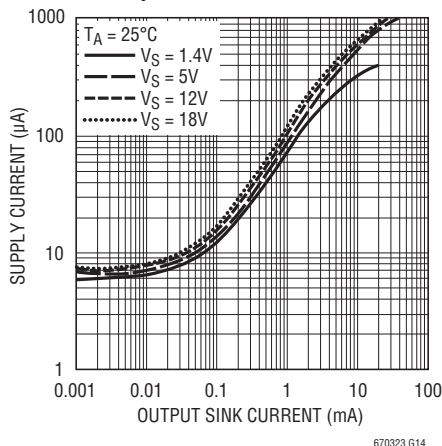
Supply Current vs Output Sink Current
