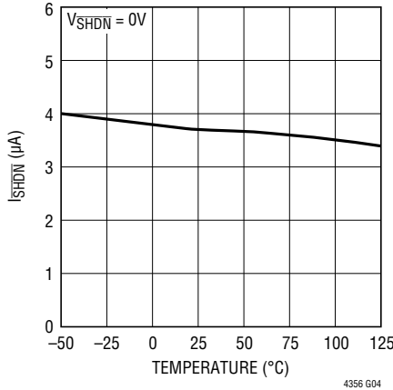
\overline{SHDN} Current vs Temperature
