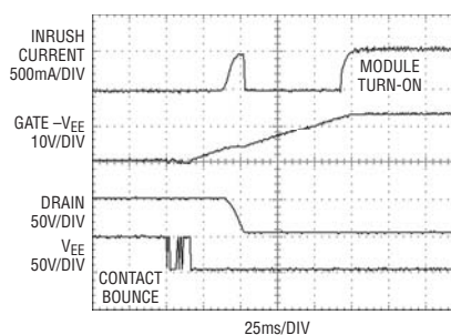
Figure 6b. Inrush Control Waveforms
