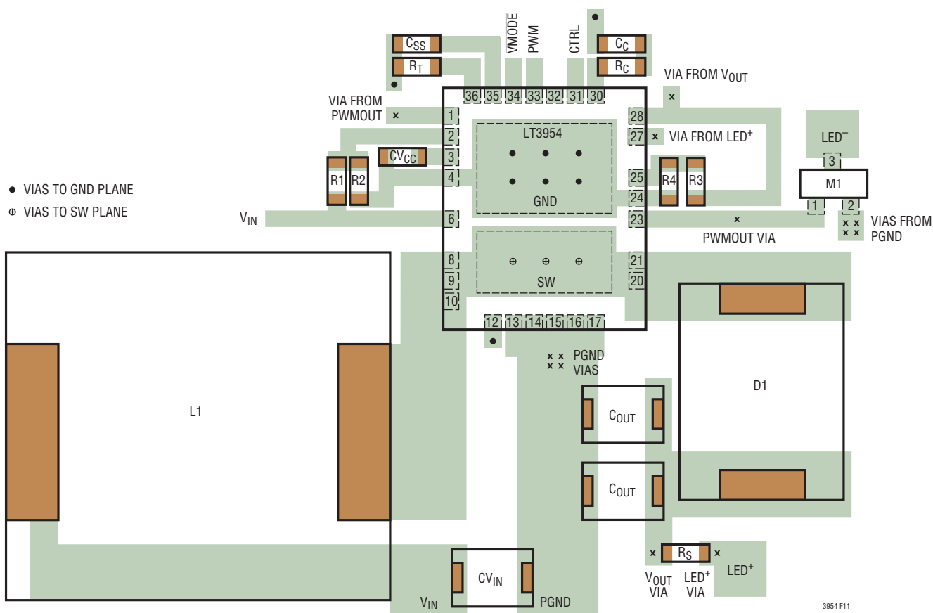
Figure 11. Boost Converter Suggested Layout
