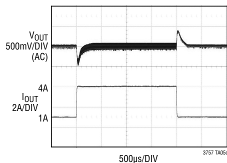
Load Step Response at V_{IN} = 12V
