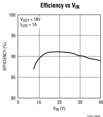
Component List: L1: WÜRTH ELEKTRONIK 744870220 M1: VISHAY SILICONIX SI7454DP D1: DIODES INC. - PDS5100 M2: VISHAY SILICONIX SI2318DS
