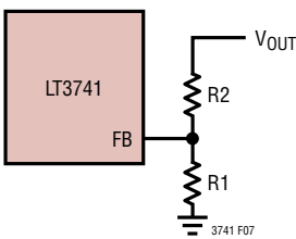
Figure 7. Output Voltage Regulation and Overvoltage Protection Feedback Connections
