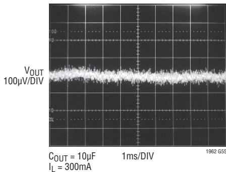
LT1962-5 10Hz to 100kHz Output Noise ( C_{\text{BYP}} = 0.01\mu\text{F} )
