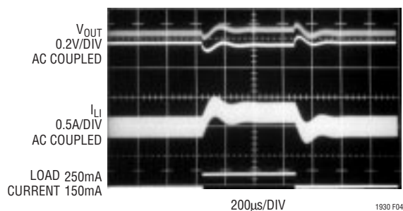
Figure 5. Transient Response of Step-Up Converter with 33μF Tantalum Output Capacitor and No Phase Lead Capacitor
