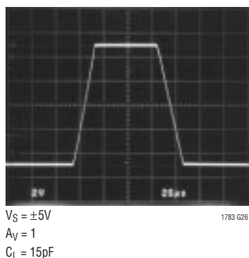
Large-Signal Response
