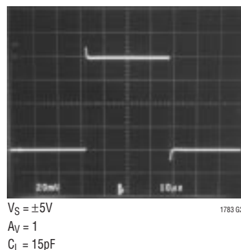
Small-Signal Response
