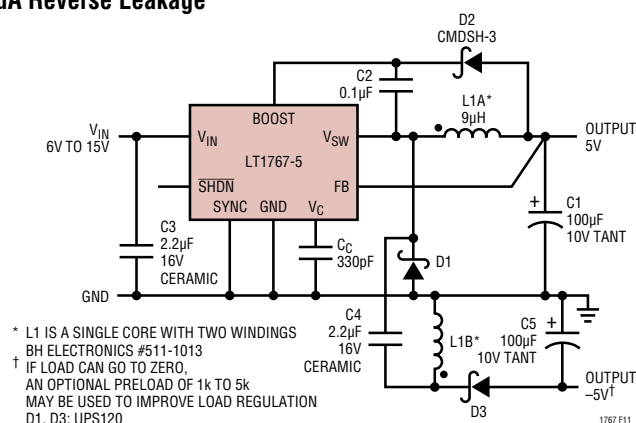
Figure 11. Dual Output SEPIC Converter
