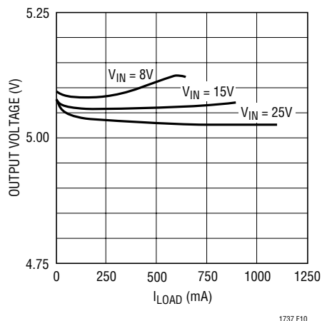
Figure 10. Output Regulation
