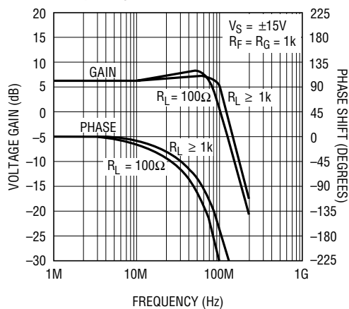
Voltage Gain and Phase vs Frequency
