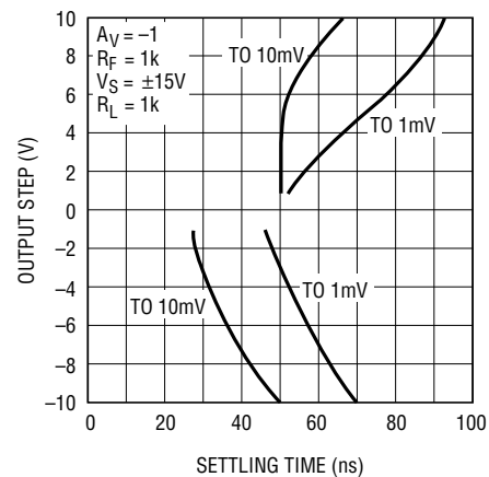
Inverting Amplifier Settling Time vs Output Step
