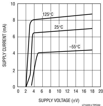
Supply Current vs Supply Voltage, V_{IN} = 0 (Operating)
