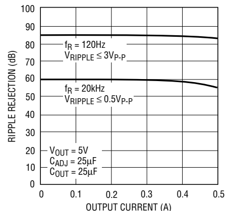
LT1086H Ripple Rejection vs Current
