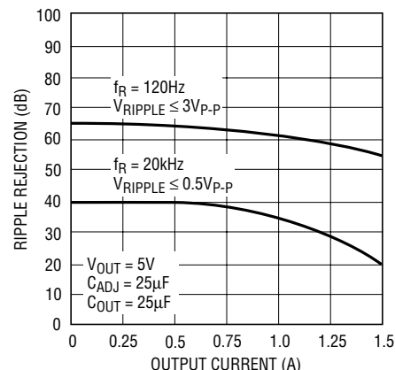
LT1086-12 Ripple Rejection vs Current
