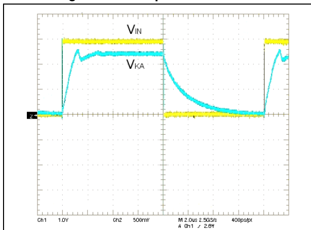
Figure 6. Startup characteristics
