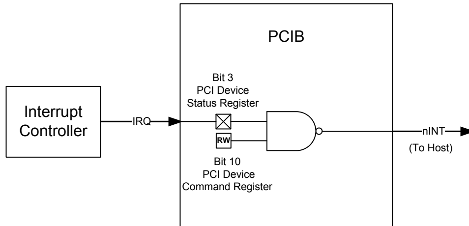
Figure 3.5 Interrupt Generation
