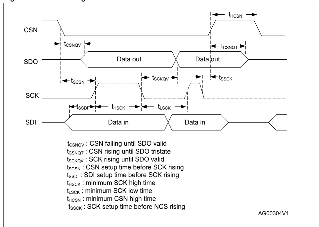
Figure 6. SPI timing
