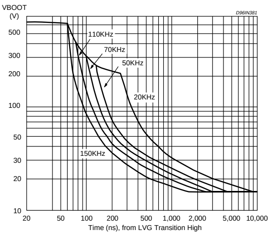
Figure 8. V boot pin SOA @ T j = 125°C
