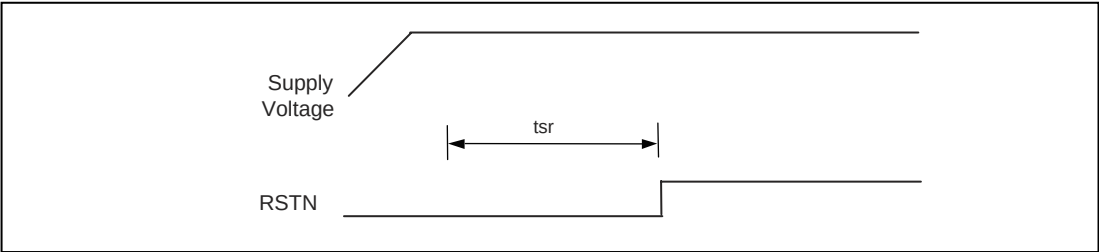
Figure 18. Reset Timing
