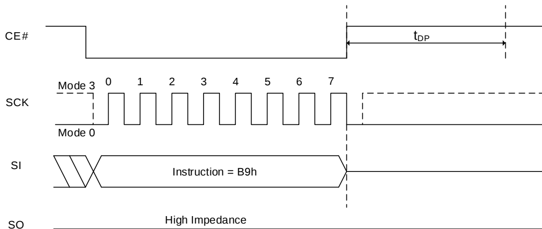
Figure 8.36 Enter Deep Power Down Mode Sequence
