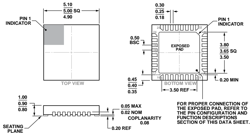
Figure 18. 32-Lead Lead Frame Chip Scale Package [LFCSP] 5 mm × 5 mm Body and 0.90 mm Package Height (HCP-32-1)
