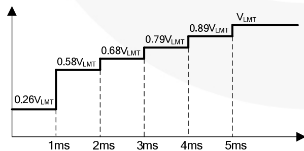
Figure 27. Soft-Start Function
