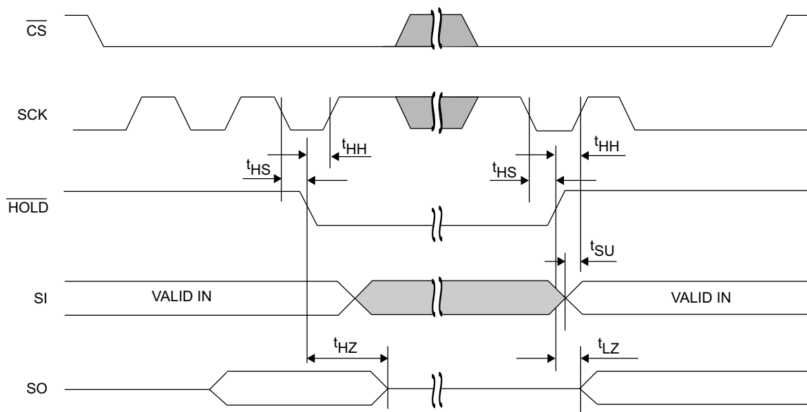
Figure 14. \overline{\text{HOLD}} Timing
