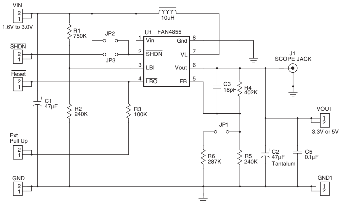
Figure 1. Test Circuit
