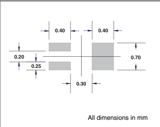
Figure 14. Footprint
