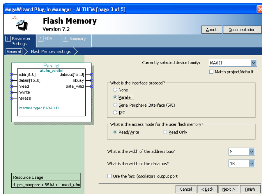
Figure 9-42. Page 3 altufm MegaWizard Plug-In Manager (Parallel)
