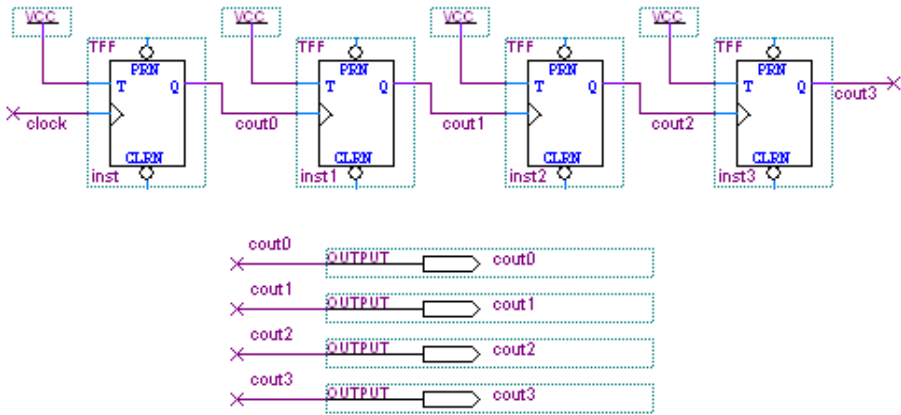
Figure 17-7. 4-Bit Counter
