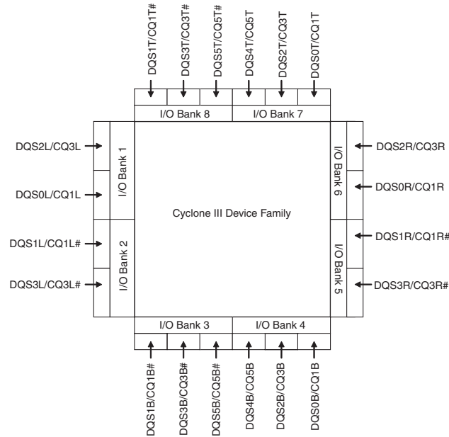
Figure 8-2. DQS, CQ, or CQ# Pins in Cyclone III Device Family I/O Banks (1)
