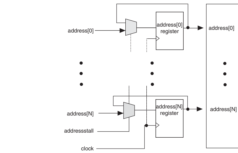
Figure 3–3. Cyclone III Device Family Address Clock Enable Block Diagram
