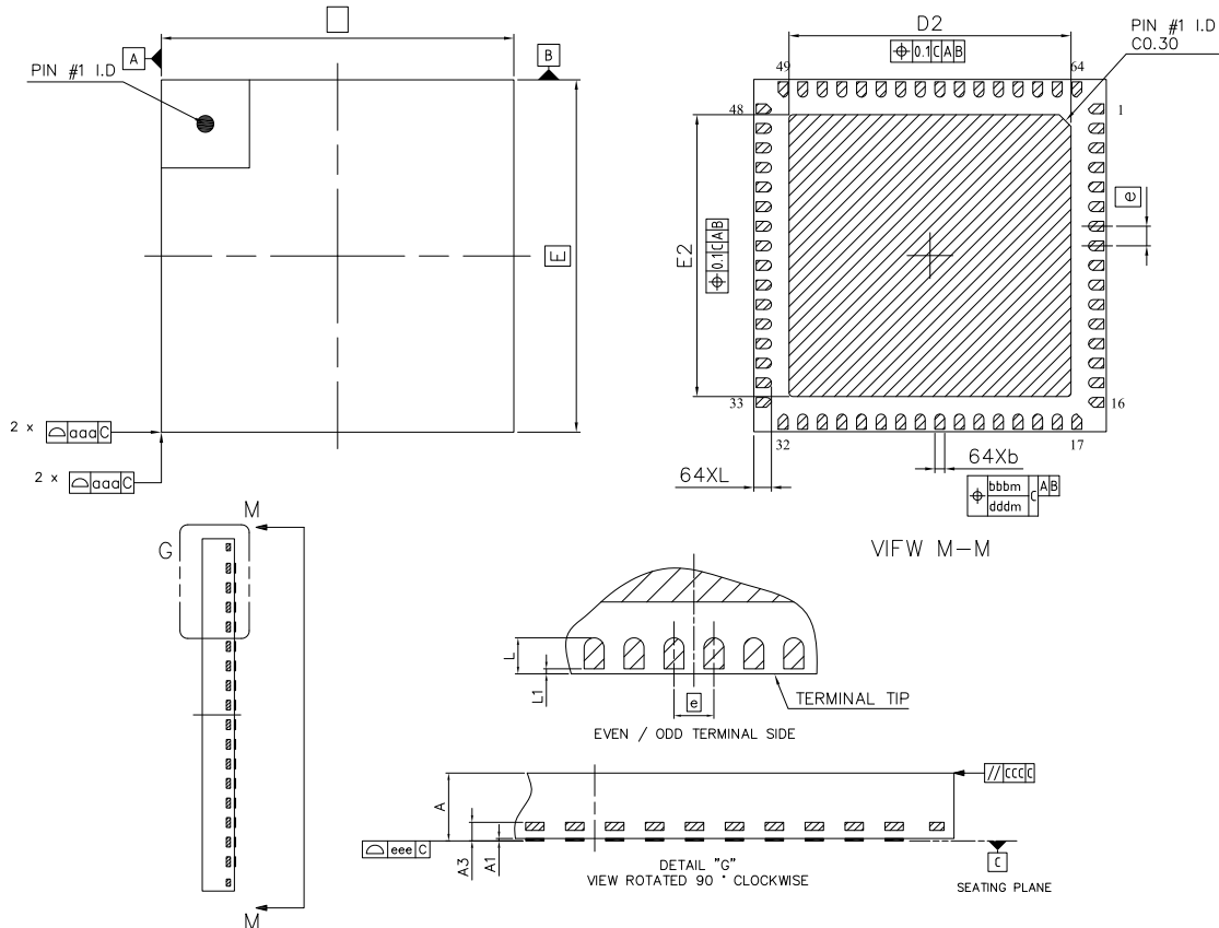
Figure 4.2. QFN64
