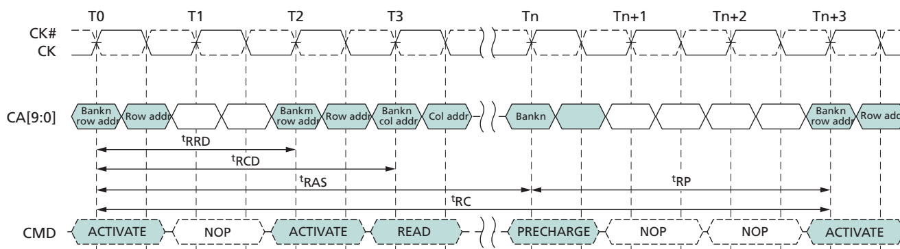
Figure 11: ACTIVATE Command
