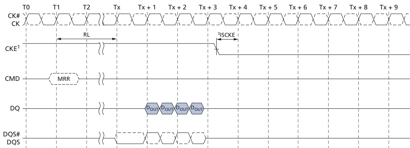
Figure 62: MRR Command to Power-Down Entry
