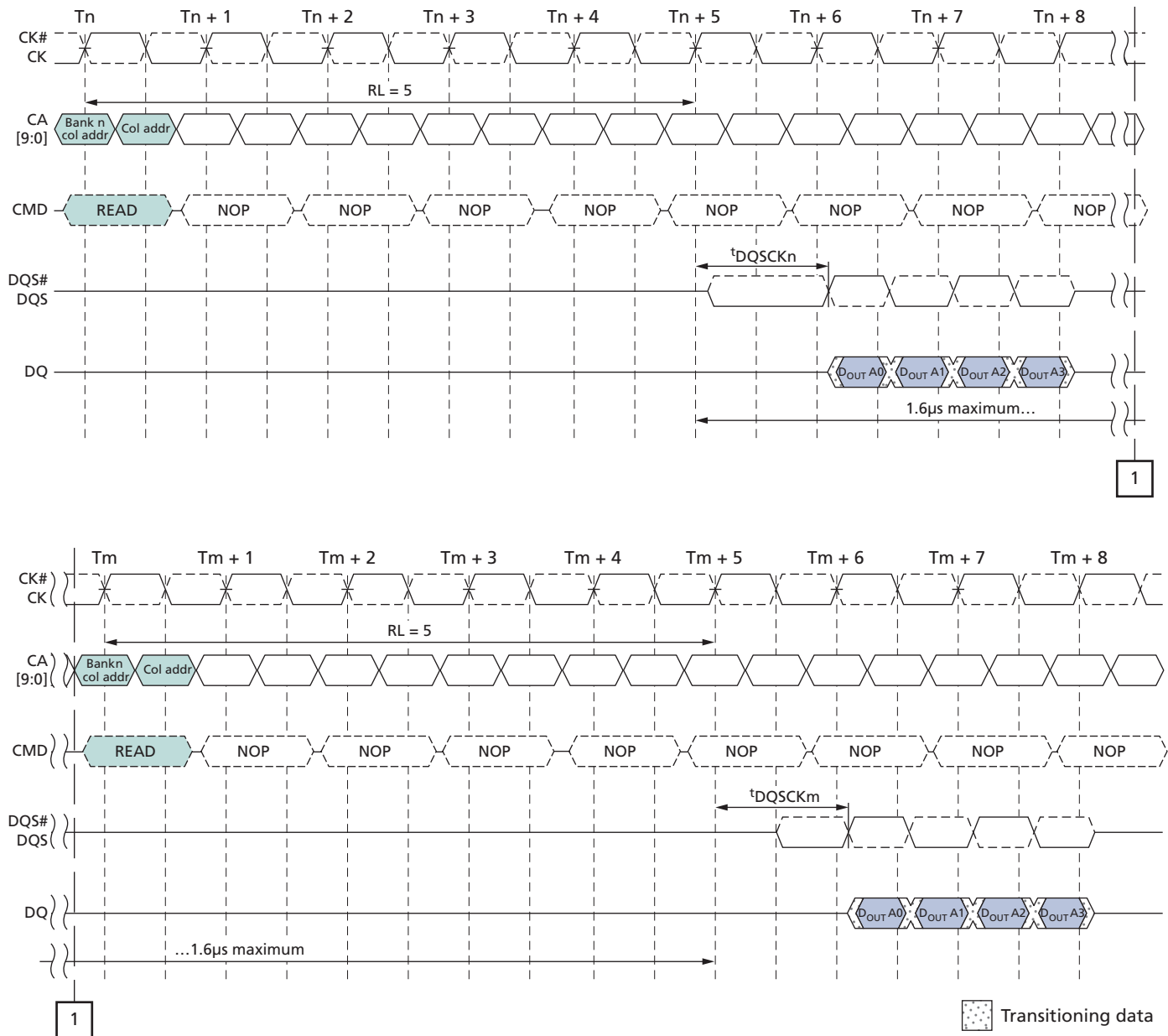
Figure 18: t_{DQSKDM} Timing
