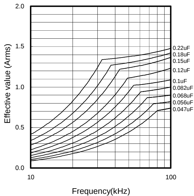
Permissible Current
