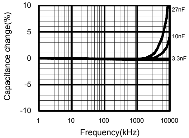
Frequency Characteristics
