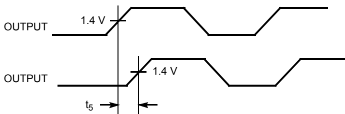
Figure 6. Output-Output Skew
