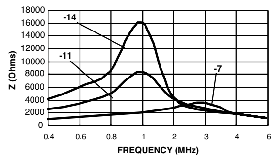
Impedance CMS2 - 7,11, & 14
