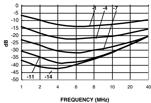
Attenuation CMS 3
