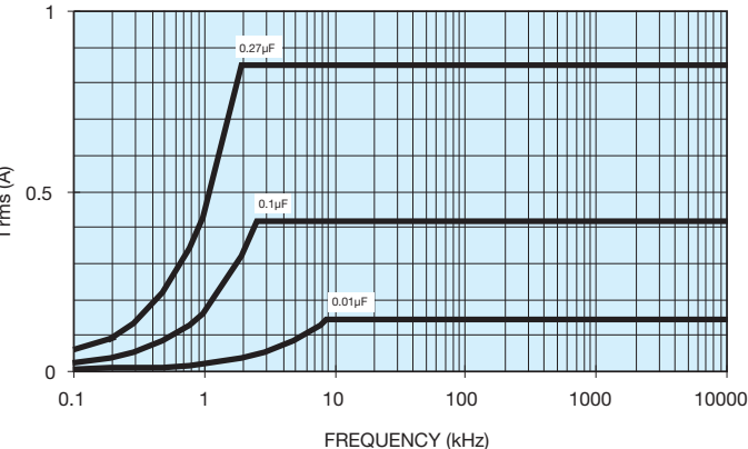
630 Vdc / 250 Vac
