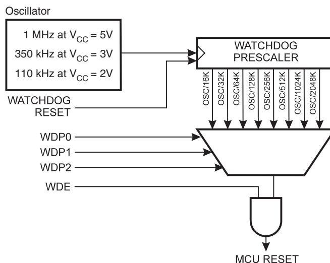
Figure 24. Watchdog Timer
