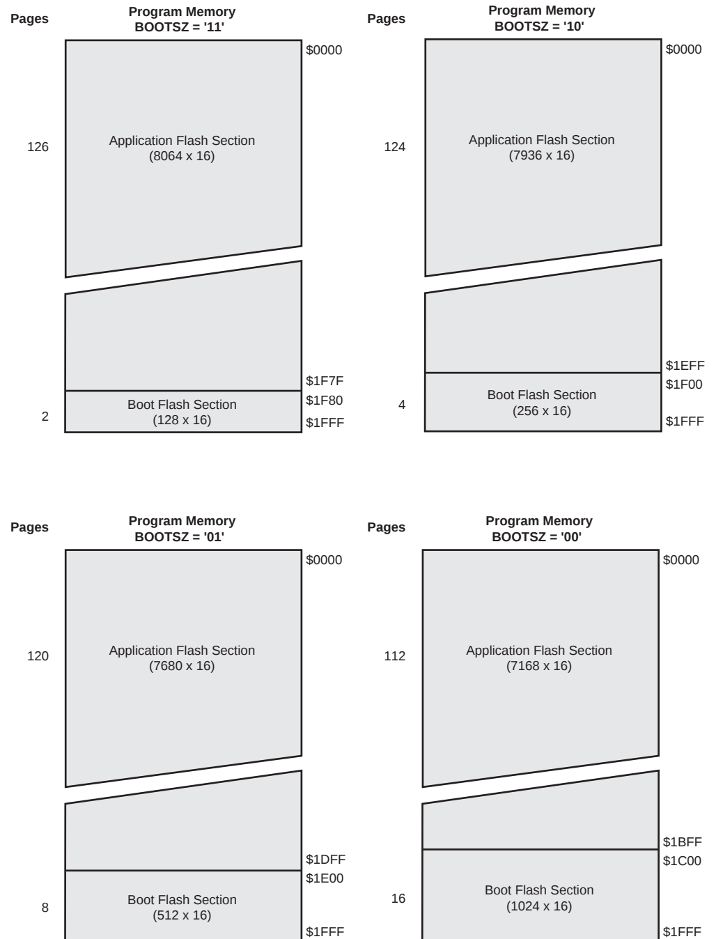
Figure 80. Memory Sections
