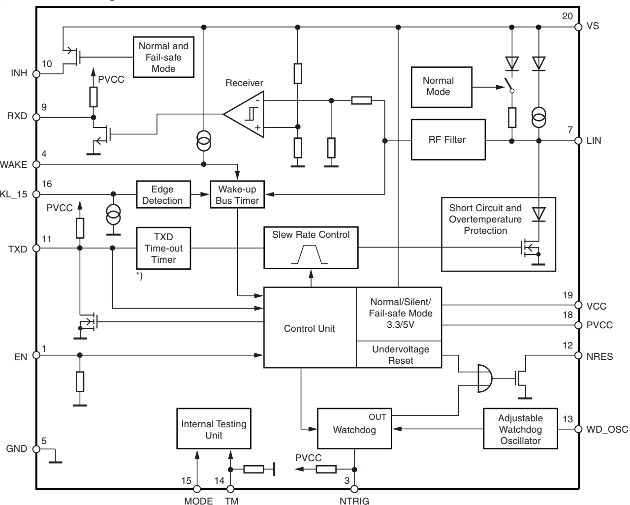
Figure 1-1. Block Diagram
