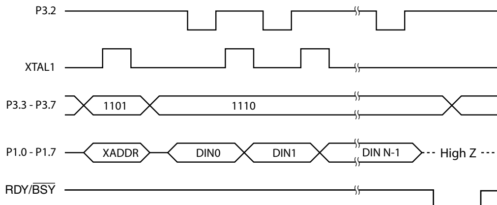
Figure 26-1. Page Write 4K Code Programming Sequence
