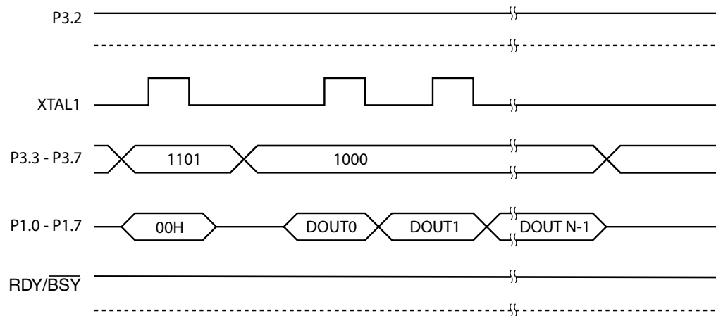
Figure 29-1. Read User Signature Row Sequence
