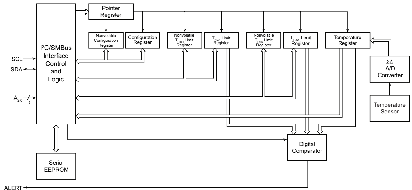
Figure 3-1. Block Diagram
