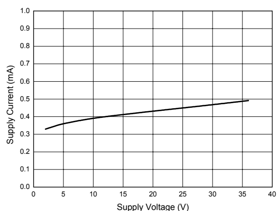
Figure 6. Supply Current
