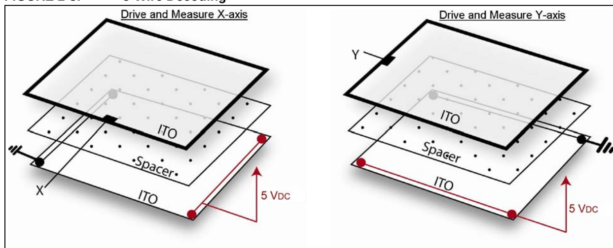
FIGURE 2-3: 5-Wire Decoding
