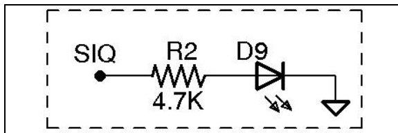
FIGURE 3-5: LED SCHEMATIC
