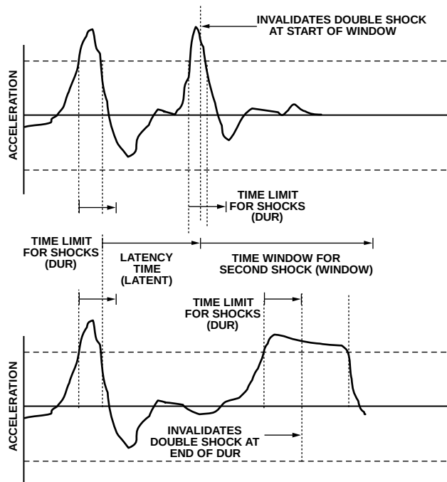
Figure 35. Shock Interrupt Function with Invalid Double Shocks
