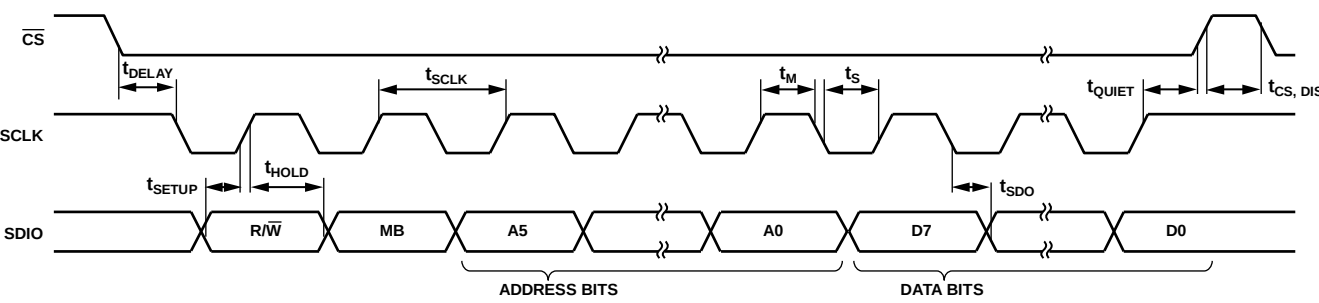
Figure 27. SPI 3-Wire Read/Write Timing Diagram
