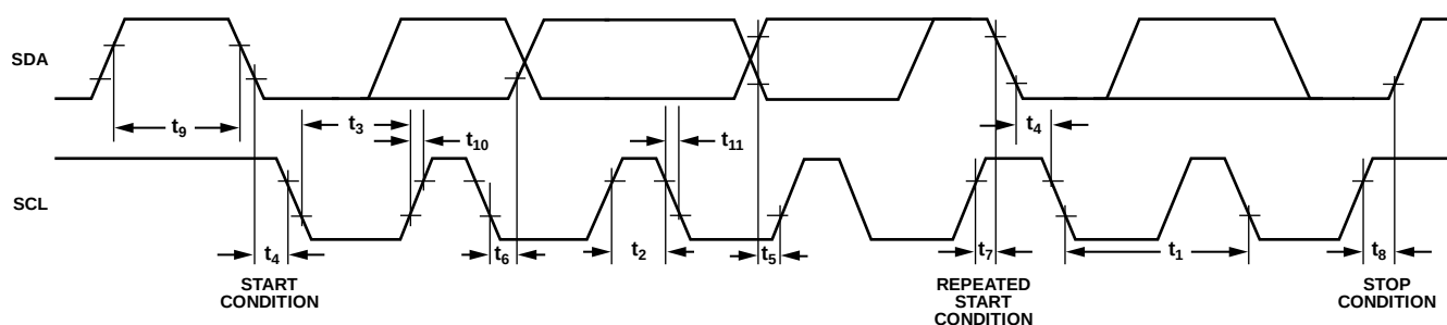
Figure 30. I 2 C Timing Diagram
