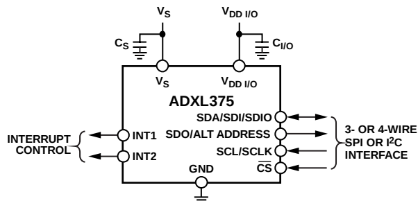
Figure 31. Application Diagram
