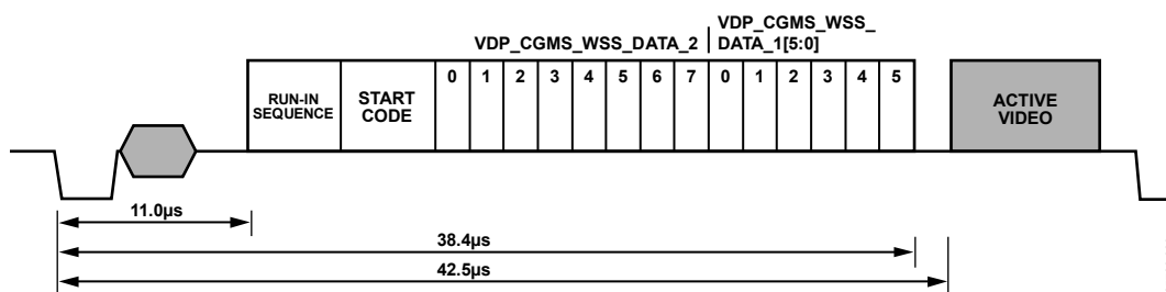
Figure 48. WSS Waveform
