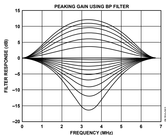
Figure 33. Peaking Filter Responses
