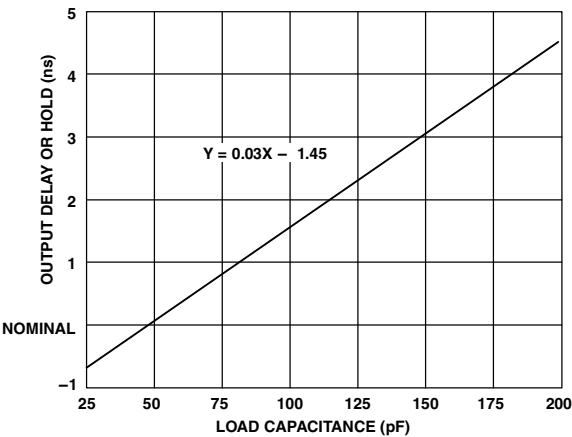
Figure 33. Typical Output Delay or Hold vs. Load Capacitance (at Maximum Case Temperature) ( V_{DD} = 5\text{ V} )
