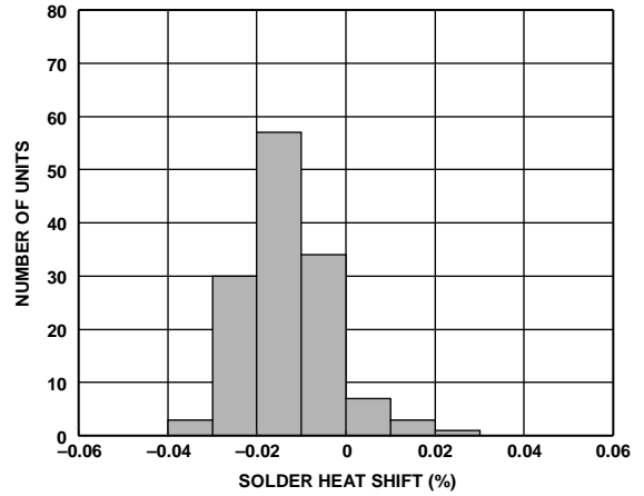
Figure 64. ADR4533 Solder Heat Resistance Shift (3 x Reflow)
