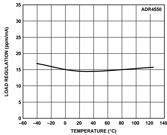
Figure 91. ADR4550 Load Regulation vs. Temperature (Sourcing)
