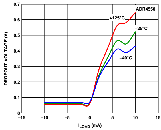
Figure 90. ADR4550 Dropout Voltage vs. Load Current
