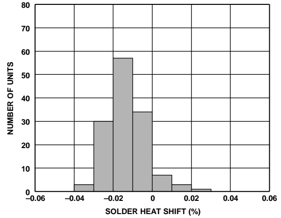
Figure 17. ADR4520 Solder Heat Resistance Shift (3 x Reflow)
