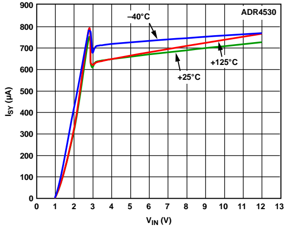
Figure 45. ADR4530 Supply Current vs. Supply Voltage
