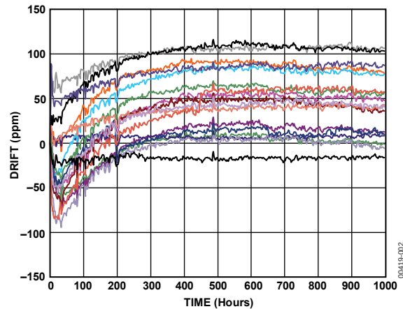
Figure 46. ADR391 Typical Long-Term Drift over 1000 Hours
